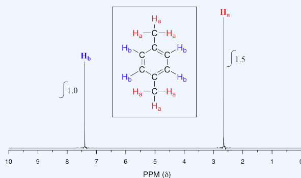
Figure 29.9m. NMR spectrum of para-xylene (IUPAC name 1,4-dimethylbenzene) (credit: Organic Chemistry: Biological Emphasis vol. 1 (page 246), CC BY-NC-SA 4.0).
