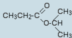
Figure 29.10i. Structure of 1-methylethyl propanoate
