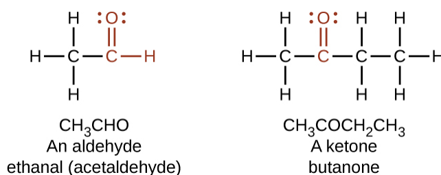
Figure 19.3c. The aldehyde is represented as -\text{CHO} whereas a ketone is represented as -\text{C}(\text{O})- or -\text{CO}- (credit: Chemistry (OpenStax) ( https://openstax.org/books/chemistry/pages/20-3-aldehydes-ketones-carboxylic-acids-and-esters ), CC BY 4.0).
