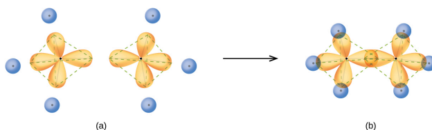
Figure 21.2l. (a) In the ethane molecule, \text{C}_2\text{H}_6 , each carbon has four sp^3 orbitals. (b) These four orbitals overlap to form seven \sigma bonds (credit: Chemistry (OpenStax), ( https://openstax.org/books/chemistry/pages/8-2-hybrid-atomic-orbitals )CC BY 4.0).
