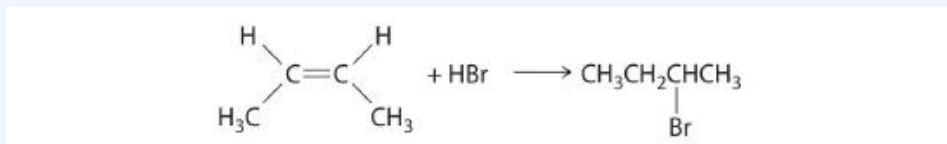
Figure 19.6j. The electrophilic addition of a HBr to 2-butene. (credit: General Chem: Principles, Patterns, and Applications (Averill), CC BY-NC-SA 3.0).
