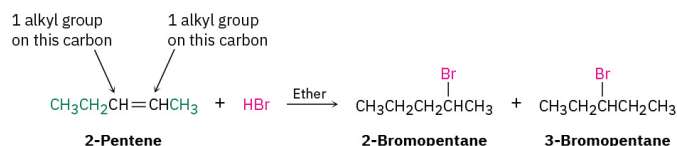
Figure 22.3e. Addition reaction when the double-bonded carbon has the same degree of substitution as shown when 2-pentene reacts with HBr. (credit: Organic Chemistry (OpenStax) , CC BY-NC-SA 4.0).
