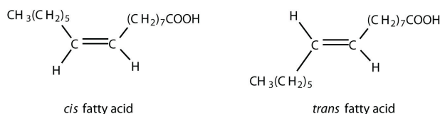
Figure 28.2b. Cis fatty acids have two H atoms on the same side of the plane of the fatty acid while trans fatty acids have the two H atoms on opposite sides (credit: Intro Chem: GOB (v. 1.0), CC BY-NC-SA 3.0).
