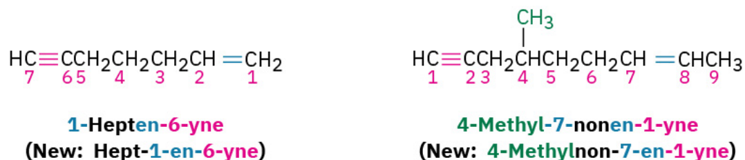
Figure 22.11. Examples of naming alkynes when numbering the double bond receives lower numbers than triple bonds. (credit: Organic Chemistry (OpenStax), CC BY-NC-SA 4.0)
