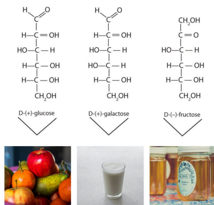
Figure 28.1h. Structures of Three Important Hexoses. Each hexose is pictured with a food source in which it is commonly found. (credit: Introduction to Chemistry: GOB (v. 1.0), CC BY-NC-SA 4.0; edited by Reva to include Photo by Nick Fewings, Photo by engin akyurt and Photo by Amelia Bartlett all under Unsplash license)
