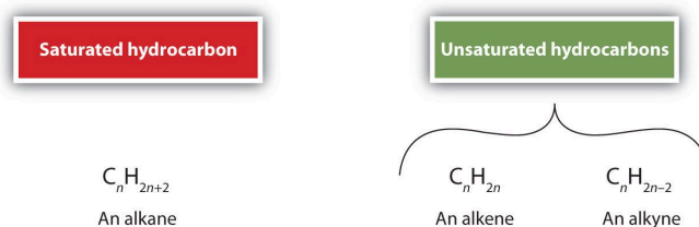
Figure 22.1a. The general formulas of alkanes, alkenes and alkynes (credit: Intro Chem: GOB (V. 1.0) , CC BY-NC-SA 3.0).
