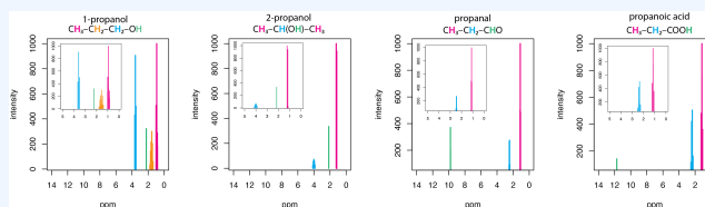
Figure 29.9k. ^1\text{H} NMR spectra for 1-propanol, 2-propanol, propanal, and propanoic acid. The full spectrum are shown using the scale at the bottom of each figure. The insets show close-ups of the NMR spectra from 0 – 5 ppm. The original data used to construct these spectra are found in the Spectral Database for Organic Compounds, SDBS [New tab] ( https://sdb.sdb.aist.go.jp/sdb/cgi-bin/direct_frame_top.cgi ). (Credit: Instrumental Analysis, CC BY-NC-SA 4.0).
