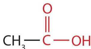
Acetic acid
