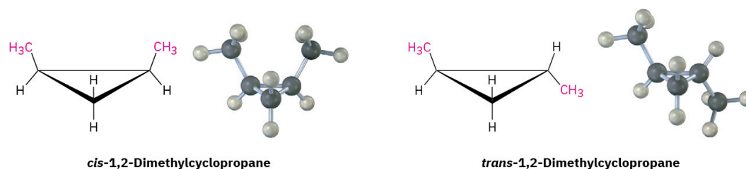
Figure 20.4l. There are two different 1,2-dimethylcyclopropane isomers, one with the methyl groups on the same face of the ring (cis) and the other with the methyl groups on opposite faces of the ring (trans). The two isomers do not interconvert (credit: Organic Chemistry (OpenStax), CC BY-NC-SA 4.0).
