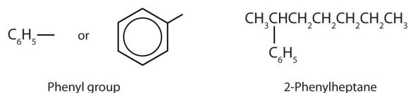
Figure 22.4g. Different ways to represent the phenyl group using a condensed structure, line structure and phenyl as a substituent (credit: Intro Chem: GOB (V. 1.0). , CC BY-NC-SA 3.0).
