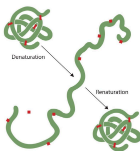
Figure 28.3s. Denaturation and Renaturation of a Protein. The denaturation (unfolding) and renaturation (refolding) of a protein is depicted. The red boxes represent stabilizing interactions, such as disulfide linkages, hydrogen bonding, and/or ionic bonds (credit: Intro Chem: GOB (v. 1.0), CC BY-NC-SA 3.0).
