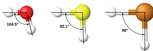
Figure 21.2q. Bond angle in \text{H}_2\text{O} ( 104.5^\circ ), \text{H}_2\text{S} ( 92.1^\circ ), and \text{H}_2\text{Te} ( 90^\circ ). (credit: Chemistry (OpenStax) ( https://openstax.org/books/chemistry/pages/8-2-hybrid-atomic-orbitals ), CC BY 4.0).
