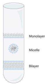
Figure 28.2m. Spontaneously Formed Polar Lipid Structures in Water: Monolayer, Micelle, and Bilayer.
