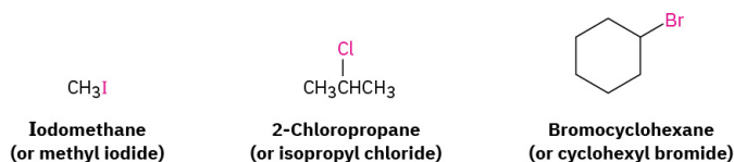
Figure 20.5i. Naming alkyl halides iodomethane, 2-chloropropane and bromocyclohexane (credit: Organic Chemistry (OpenStax) ( https://openstax.org/books/organic-chemistry/pages/10-1-names-and-structures-of-alkyl-halides ), CC BY-NC-SA 4.0).
