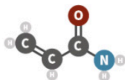
ACRYLAMIDE
