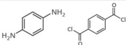
MONOMERS: 1,4-PHENYLENE-DIAMINE & TEREPHTHALOYL CHLORIDE
