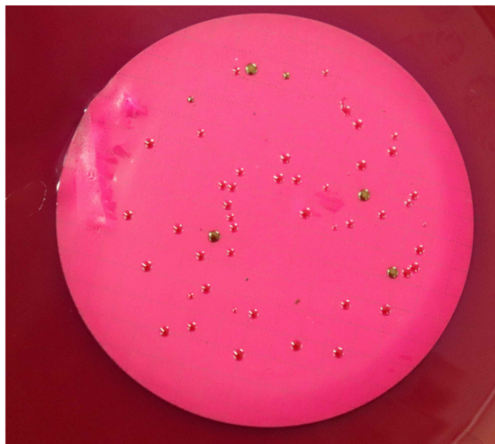
Figure 9.1. Water test media detects coliforms based on lactose fermentation. Coliforms on lactose broth and BGLB make gas (see in the tube on the left). E. coli on differential coliform agar (DC) are metallic green or gold (see the plate on the right).
