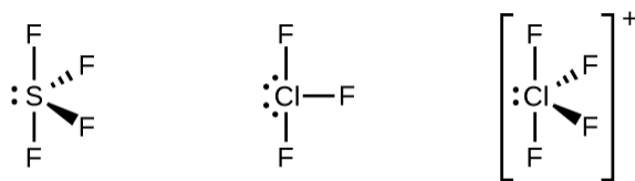
Figure 21.2m. The three compounds pictured exhibit sp^3d hybridization in the central atom and a trigonal bipyramidal form. \text{SF}_4 and \text{ClF}_4^+ have one lone pair of electrons on the central atom, and \text{ClF}_3 has two lone pairs giving it the T-shape shown (credit: Chemistry (OpenStax) ( https://openstax.org/books/chemistry/pages/8-2-hybrid-atomic-orbitals ), CC BY 4.0).
