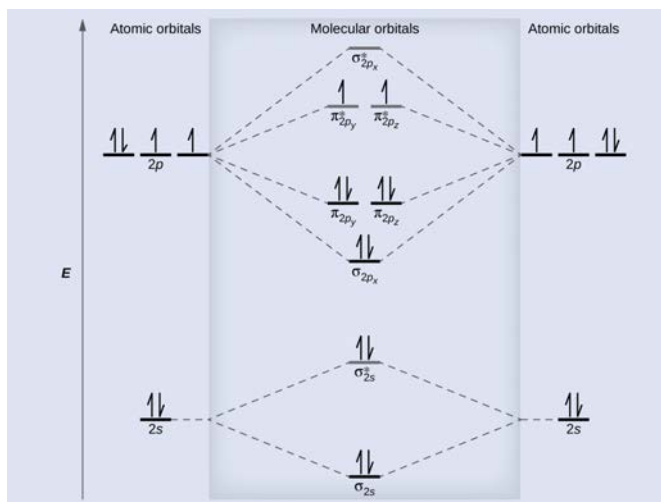
Figure 21.4n. The molecular orbital energy diagram for O_2 predicts two unpaired electrons (credit: Chemistry (OpenStax) ( https://openstax.org/books/chemistry/pages/8-4-molecular-orbital-theory ), CC BY 4.0).
