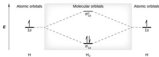
Figure 21.4j. The molecular orbital energy diagram predicts that \text{H}_2 will be a stable molecule with lower energy than the separated atoms (credit: Chemistry (OpenStax) ( https://openstax.org/books/chemistry/pages/8-4-molecular-orbital-theory ), CC BY 4.0).
