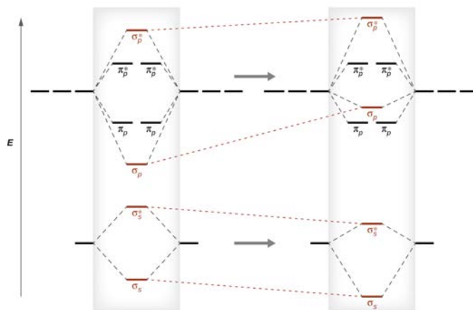
Figure 21.4m. Without mixing, the MO pattern occurs as expected, with the \sigma_p orbital lower in energy than the \sigma_p orbitals. When s-p mixing occurs, the orbitals shift as shown, with the \sigma_p orbital higher in energy than the \pi_p orbitals (credit: Chemistry (OpenStax) ( https://openstax.org/books/chemistry/pages/8-4-molecular-orbital-theory ), CC BY 4.0).
