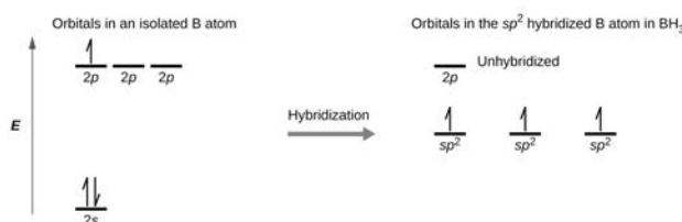
Figure 21.2h. In an isolated B atom, there are one 2s and three 2p valence orbitals. When boron is in a molecule with three regions of electron density, three of the orbitals hybridize and create a set of three sp^2 orbitals and one unhybridized 2p orbital. The three half-filled hybrid orbitals each overlap with an orbital from a hydrogen atom to form three \sigma bonds in BH_3 (credit: Chemistry (OpenStax), ( https://openstax.org/books/chemistry/pages/8-2-hybrid-atomic-orbitals )CC BY 4.0).
