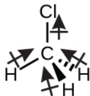
Figure 11.6p The \text{CH}_3\text{Cl} structure has a tetrahedral shape and represents a polar molecule (credit: Chemistry (OpenStax) , CC BY 4.0).
